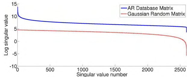
Figure 1. The log of the singular values of the data matrix A calculated using the AR data set, and for comparison, of a matrix of the same size with elements sampled from \mathcal{N}(0, 1) .
