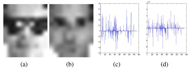
Figure 6. Prediction on downsampled AR faces with size 13 \times 10 . (a) test face. (b) predicted test face by \ell_1 and \ell_{1r} . (c) estimated coefficient \alpha via \ell_1 . The coefficient achieved by \ell_{1r} is very similar to (c), thus it is not presented here. (d) The difference of the estimated coefficients by \ell_1 and \ell_{1r} . The difference is only in O(10^{-4}) .
